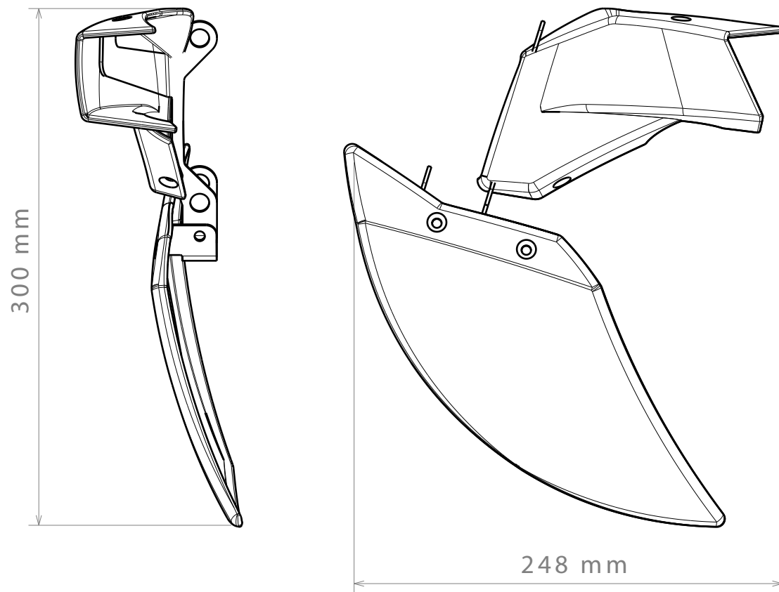
RIGHT BRAKE COOLER
