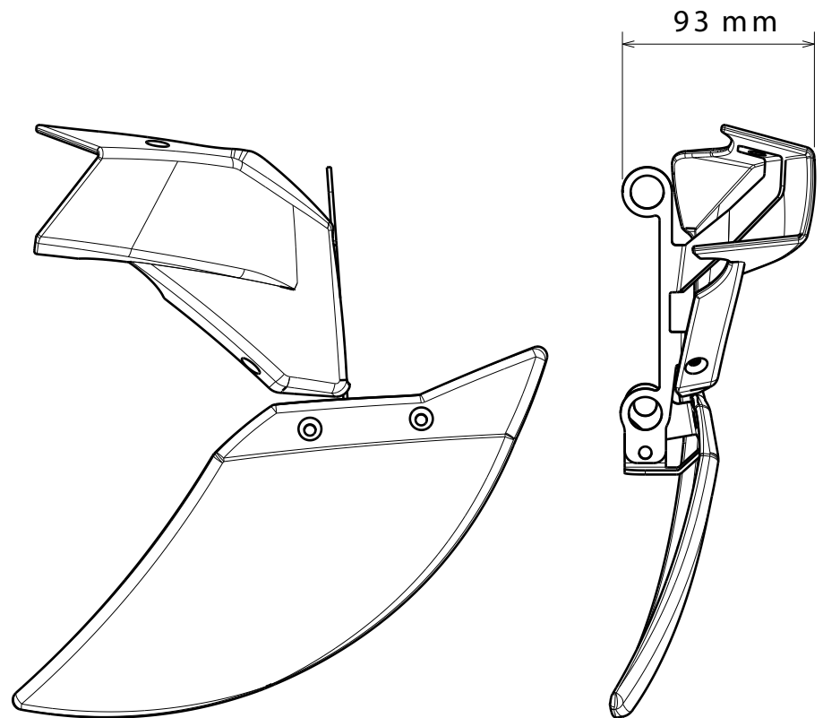
LEFT BRAKE COOLER
