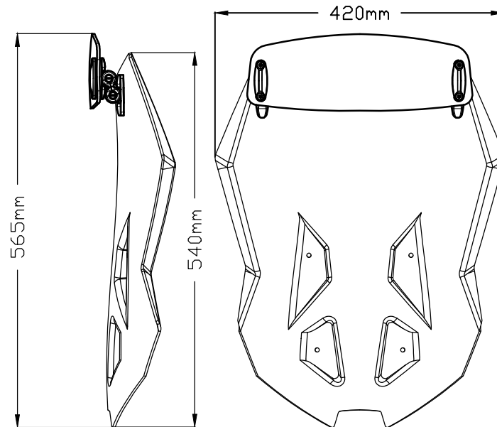
TOURING SCREEN WITH VISOR AT UPPER POSITION
