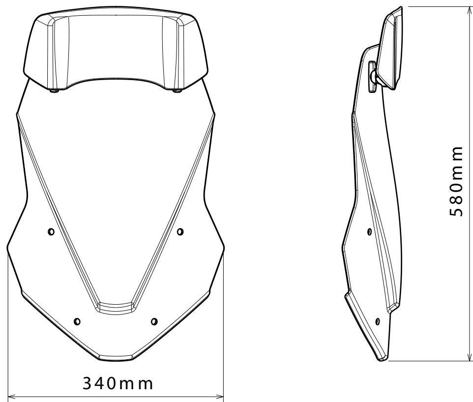
TOURING SCREEN WITH VISOR AT HIGHER POSITION
