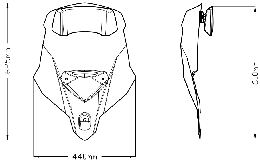
TOURING SCREEN WITH VISOR AT UPPER POSITION
