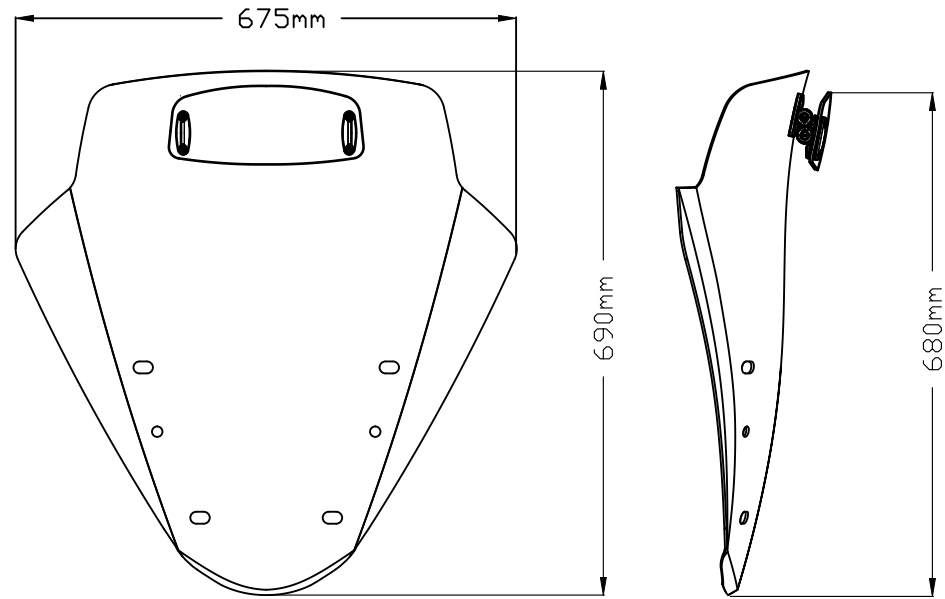
TOURING SCREEN WITH VISOR AT UPPER POSITION
