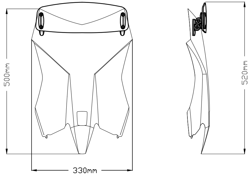
TOURING SCREEN WITH VISOR AT UPPER POSITION
