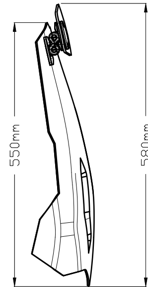
TOURING SCREEN WITH VISOR AT UPPER POSITION
